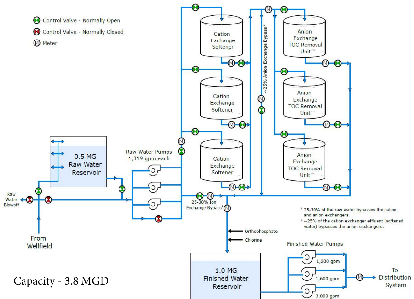
MCAS New River WTP Schematic
